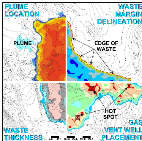
Figure 4 TDEM map of underground storage tank locations (blue to red are low to high millivolts, respectively).
