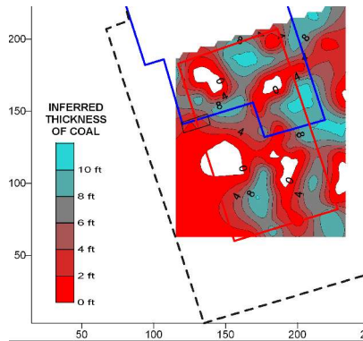
Figure 10 Plan map of interpreted coal thickness in an underground mine (in feet).
