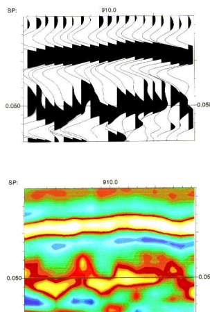
Figure 9 Conventional reflection seismic profile (top) and amplitude profile (bottom) of coal-mine voids (vertical scale in milliseconds; horizontal scale, 3 meters between records).
