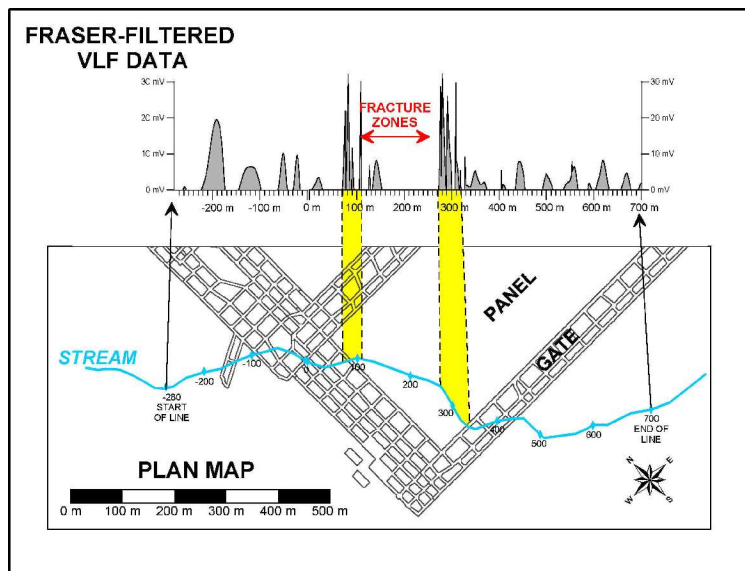
Figure 7 VLF map showing long-wall mining-induced fractures in a stream bank (from Hutchinson and Barta, 2002).
