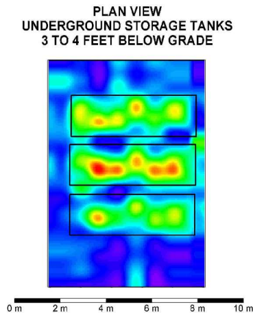
Figure 3 Average amplitude map of 3 underground storage tanks from three-dimensional GPR survey
