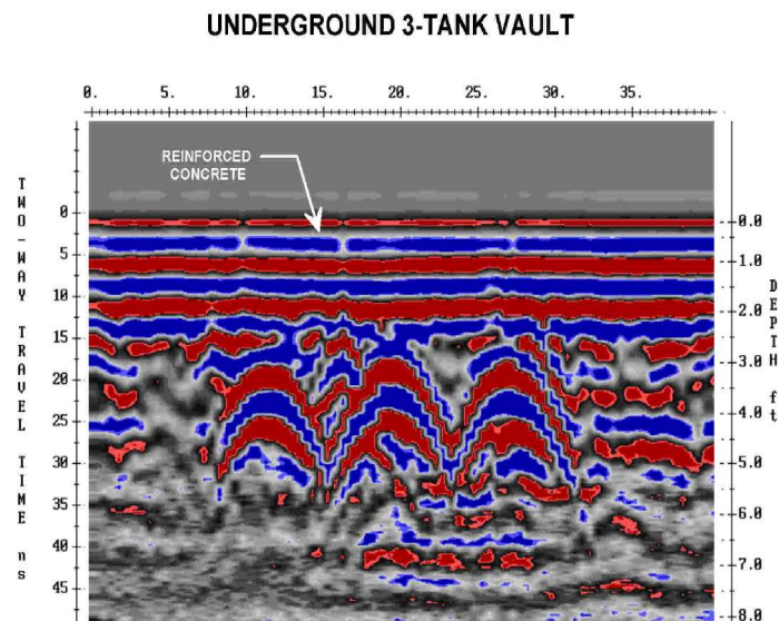
Figure 2 Ground penetrating radar profile of 3 underground storage tanks (horizontal scale in feet).
