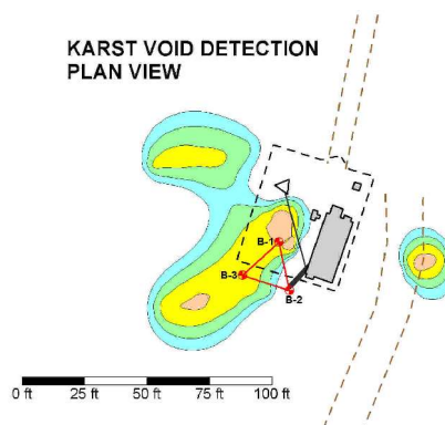
Figure 11 Electrical imaging profile of a karst void (no vertical exaggeration, in feet)
