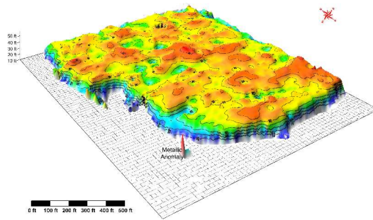
Figure 6 Processed terrain conductivity data, showing an inferred depth of waste.
